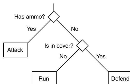
Figure 7.13 Decision tree before ID4
