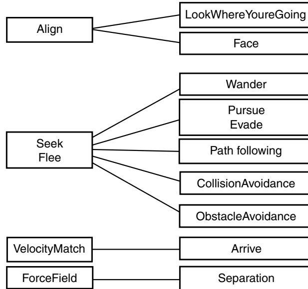
Figure 3.29 Steering family tree
