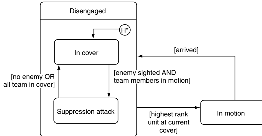
Figure 6.27 State machines for emergent fire team behavior
