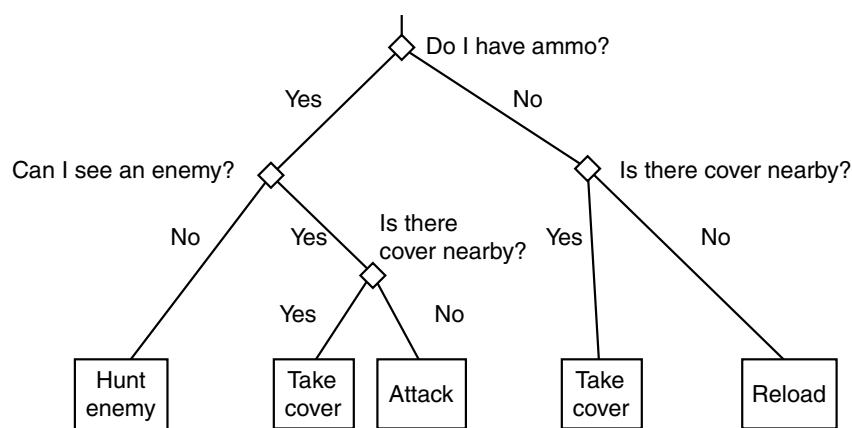
Figure 6.6 Tactical information in a decision tree
