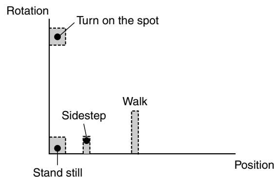
Figure 4.53 Example of position ranges for animations
