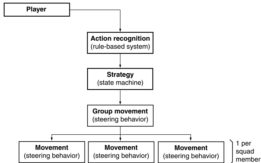
Figure 6.25 A multi-tier AI involving the player
