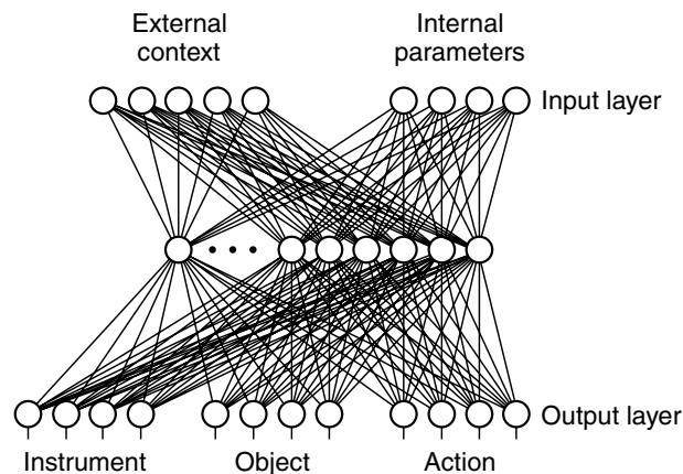
Figure 13.1 Neural network architecture for creature-teaching games
