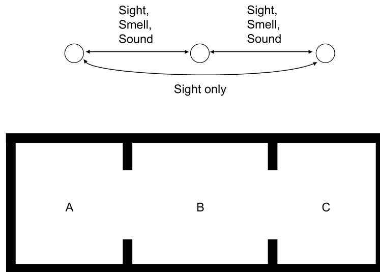
Figure 10.10 The sight sense graph
