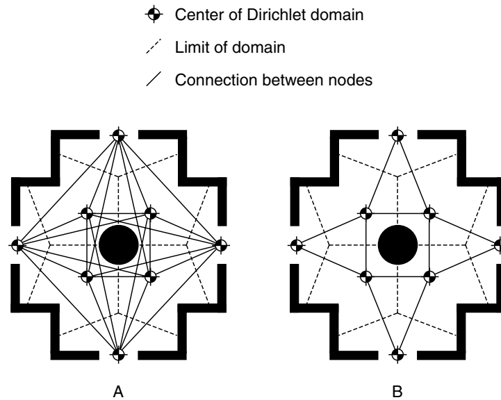
Figure 11.2 A visibility-based graph and its post-processed form
