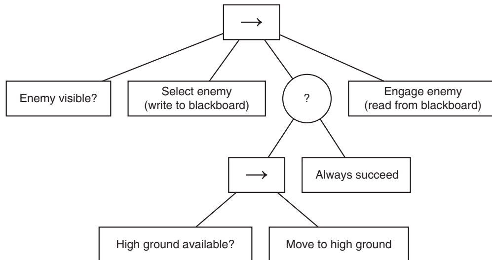
Figure 5.36 A behavior tree communicating via blackboard
