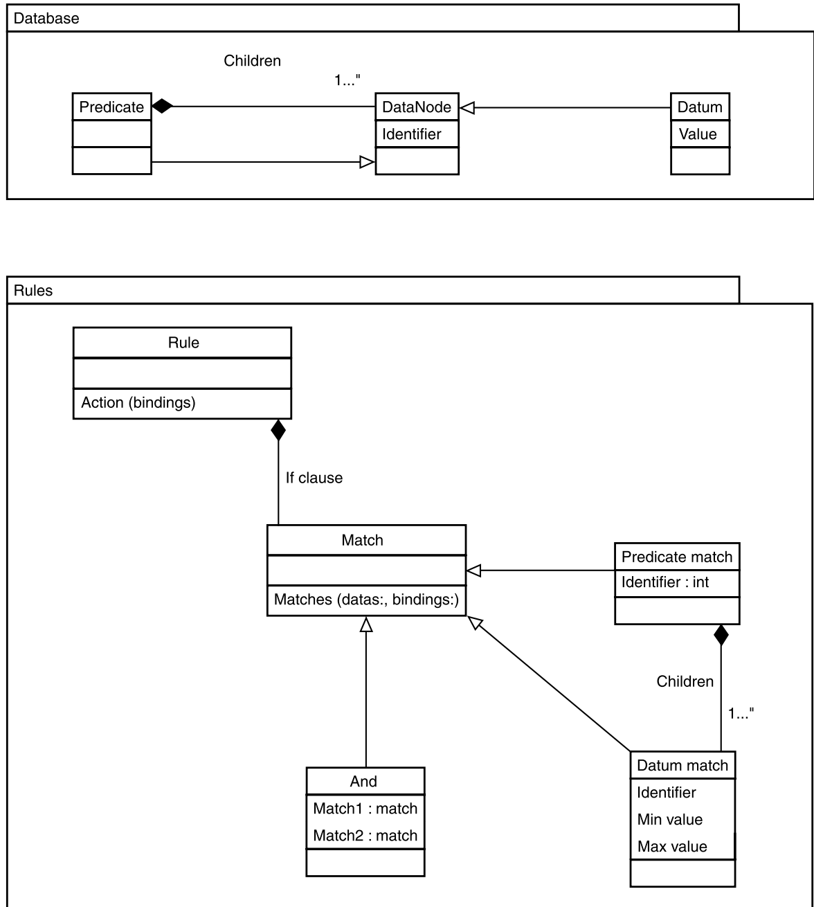
Figure 5.47 UML of the matching system
