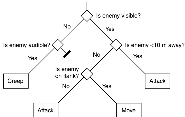
Figure 5.3 A decision tree
