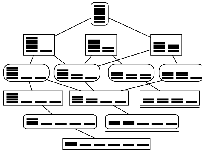
Figure 8.3 The game tree of 7-Split-Nim
