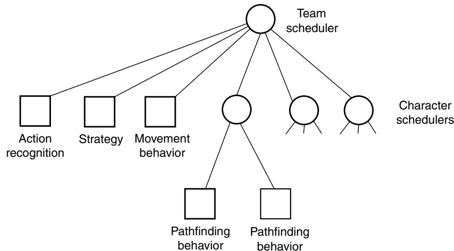
Figure 6.26 A hierarchical scheduling system for multi-tier AI
