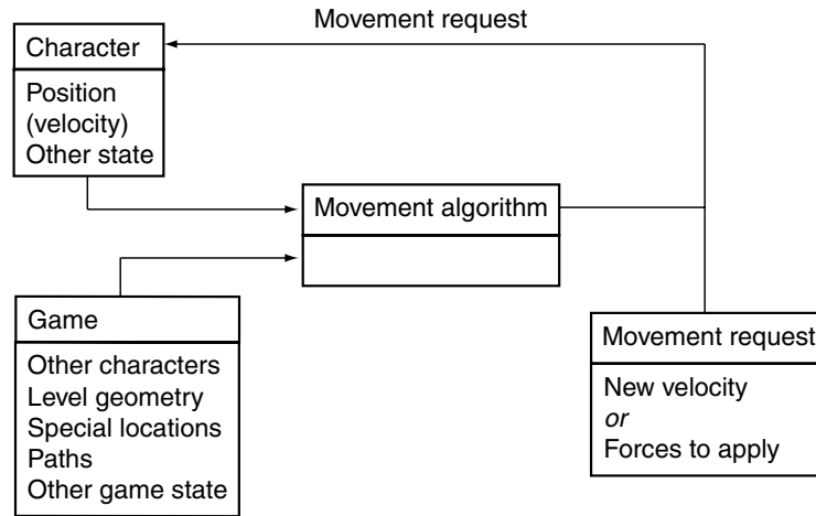
Figure 3.2 The movement algorithm structure
