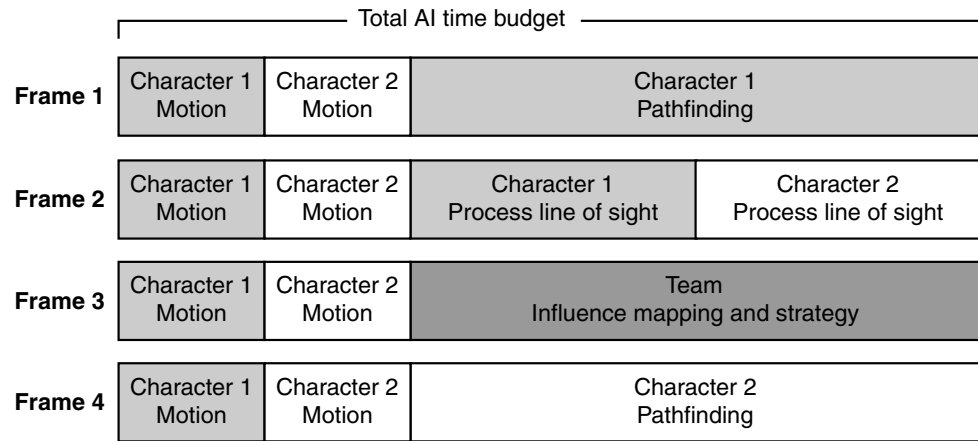
Figure 9.1 AI slicing
