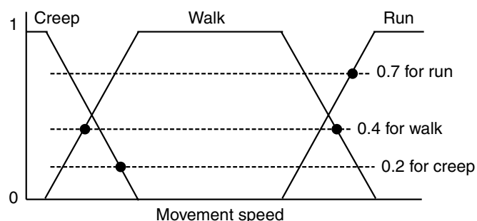
Figure 5.40 Impossible defuzzification
