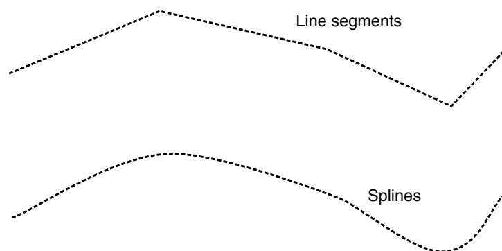
Figure 3.18 Path types
