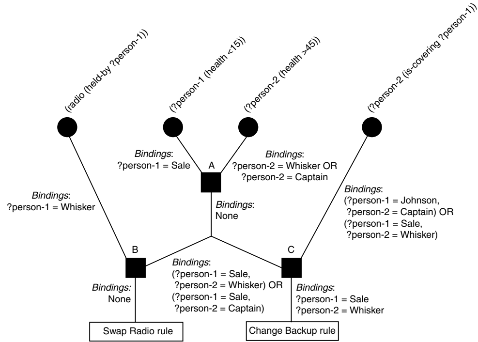
Figure 5.52 Rete after-update
