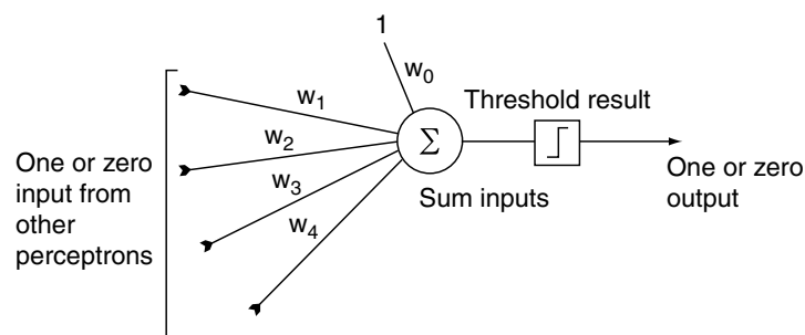
Figure 7.19 Perceptron algorithm
