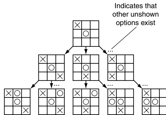
Figure 8.1 Tic-Tac-Toe game tree
