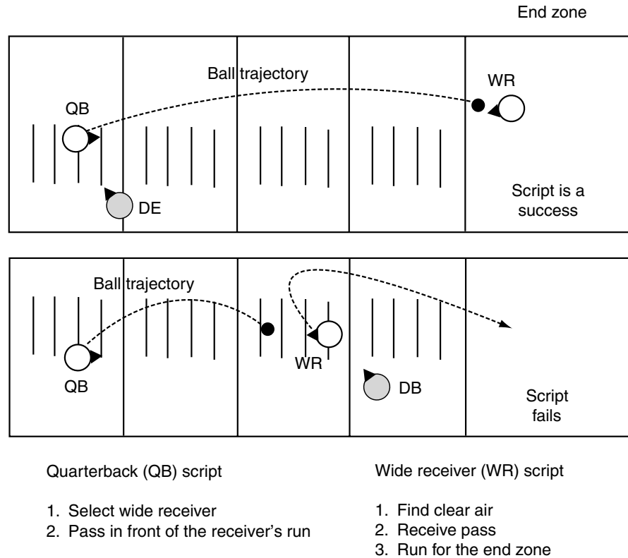
Figure 6.28 An action sequence needing timing data
