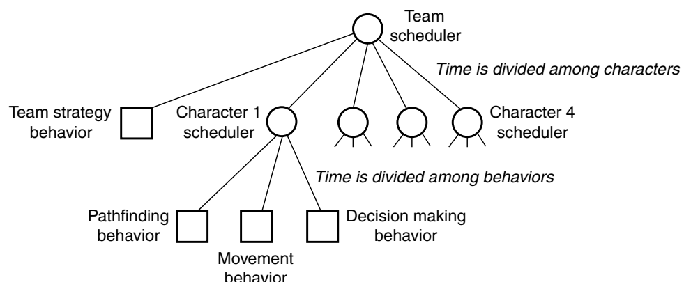
Figure 9.5 Behaviors in a hierarchical scheduling system
