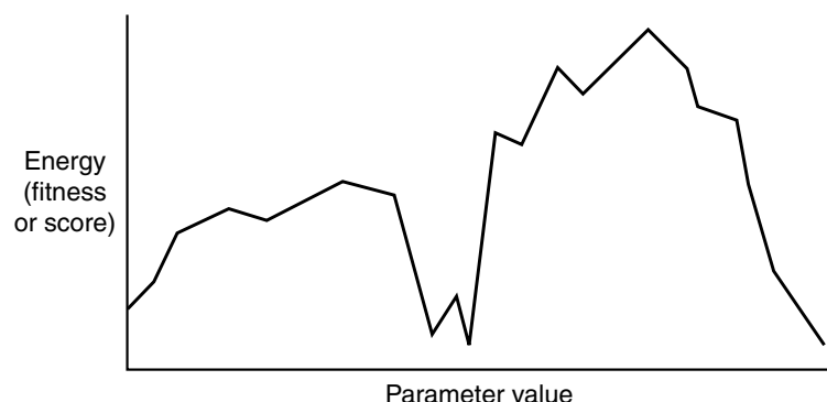
Figure 7.1 The energy landscape of a one-dimensional problem
