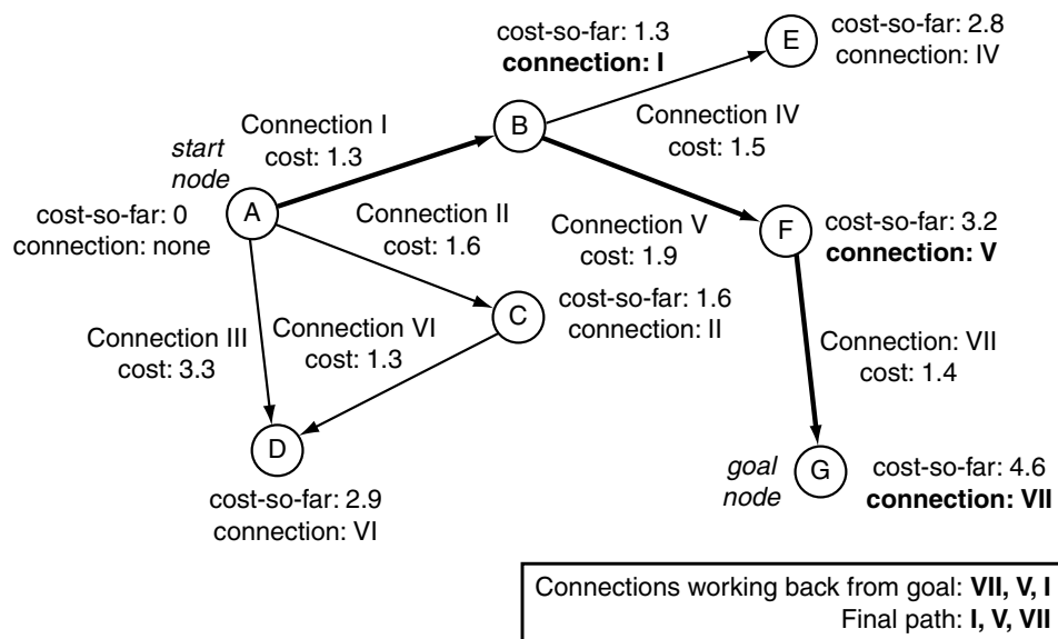
Figure 4.11 Following the connections to get a plan
