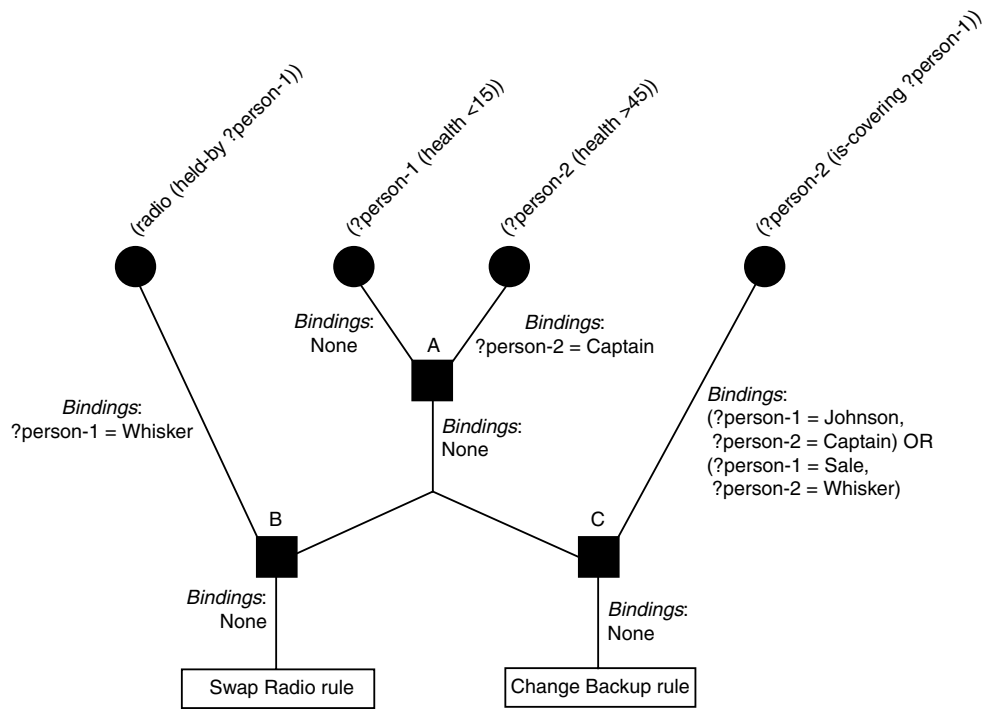
Figure 5.51 Rete in mid-update
