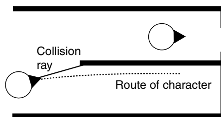
Figure 3.37 Long distance failure in a steering behavior
