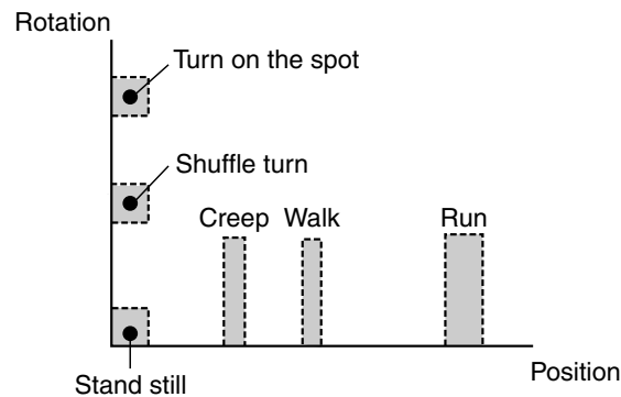
Figure 4.51 Position diagram for allowed animations
