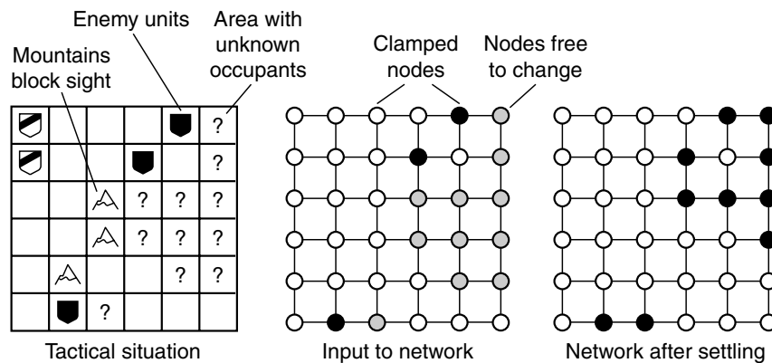
Figure 7.25 Influence mapping with Hebbian learning
