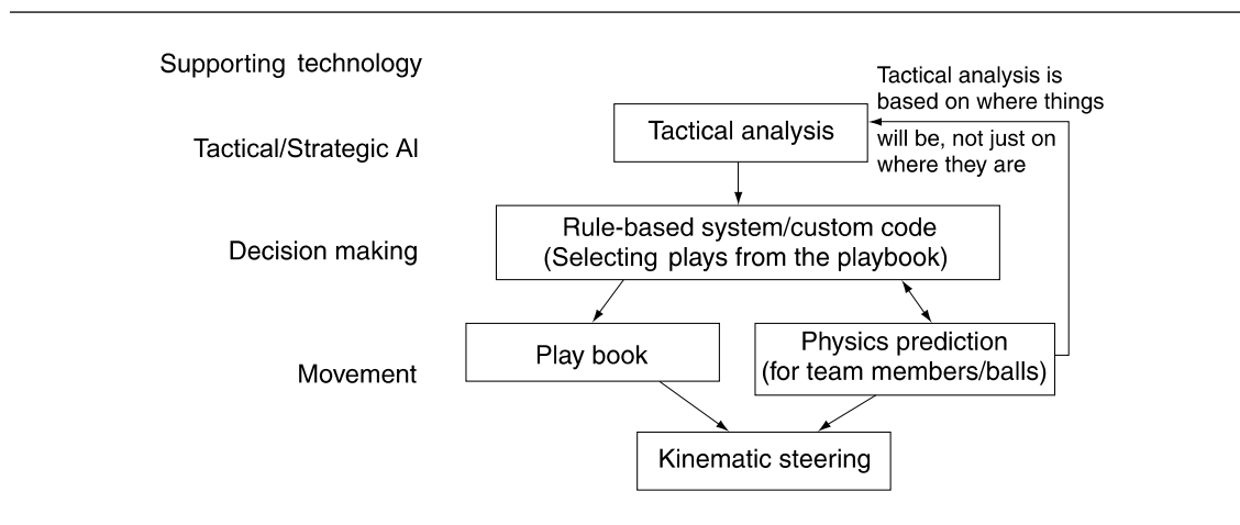
Figure 12.6 AI architecture for sports games
