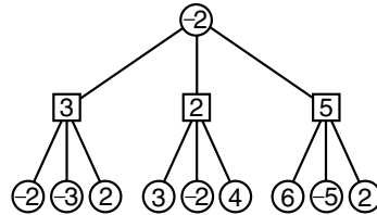
Figure 8.8 Negamax values bubbled up a tree
