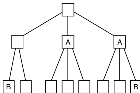
Figure 5.45 Why to replace transposition entries lower down
