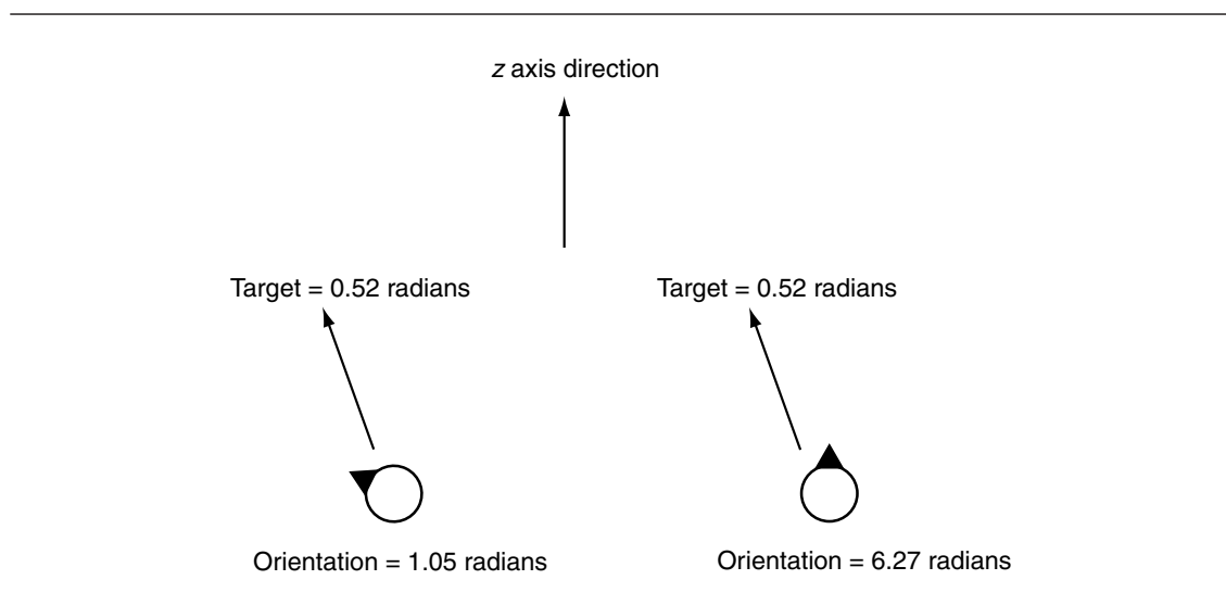
Figure 3.10 Aligning over a 2\pi radians boundary
