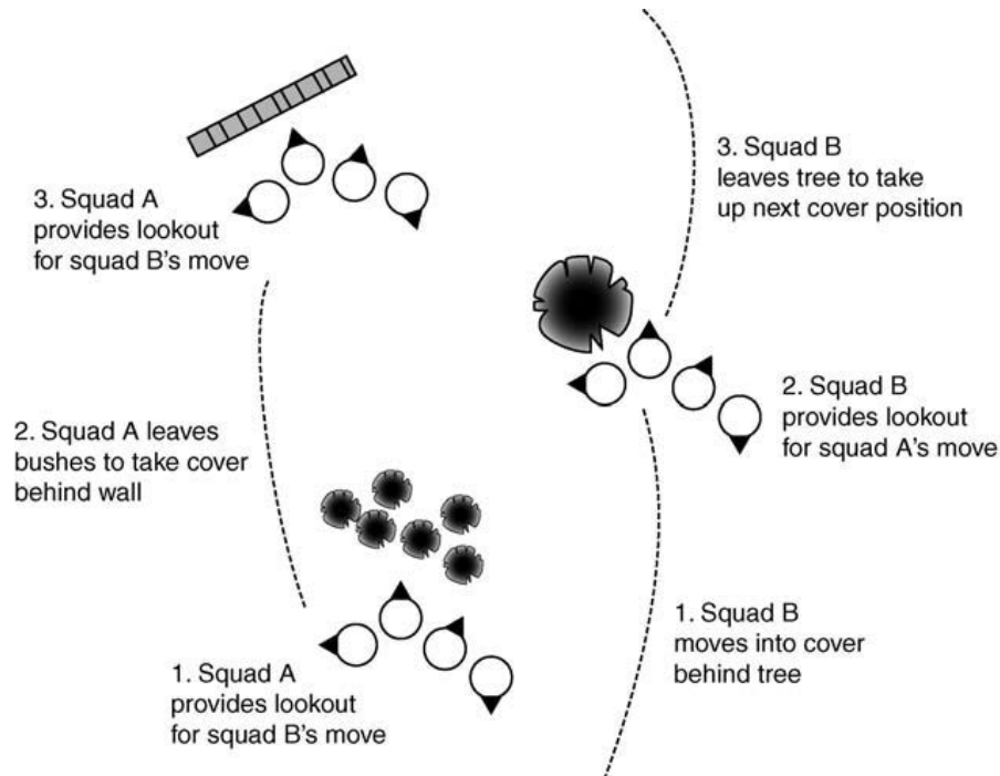
Figure 3.64 Bounding overwatch
