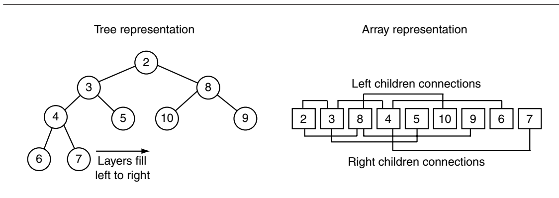
Figure 4.15 Priority heap
