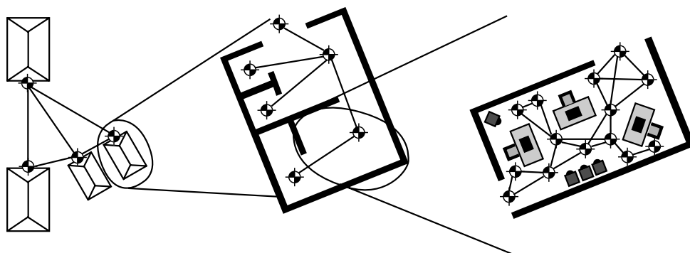
Figure 4.37 Hierarchical nodes
