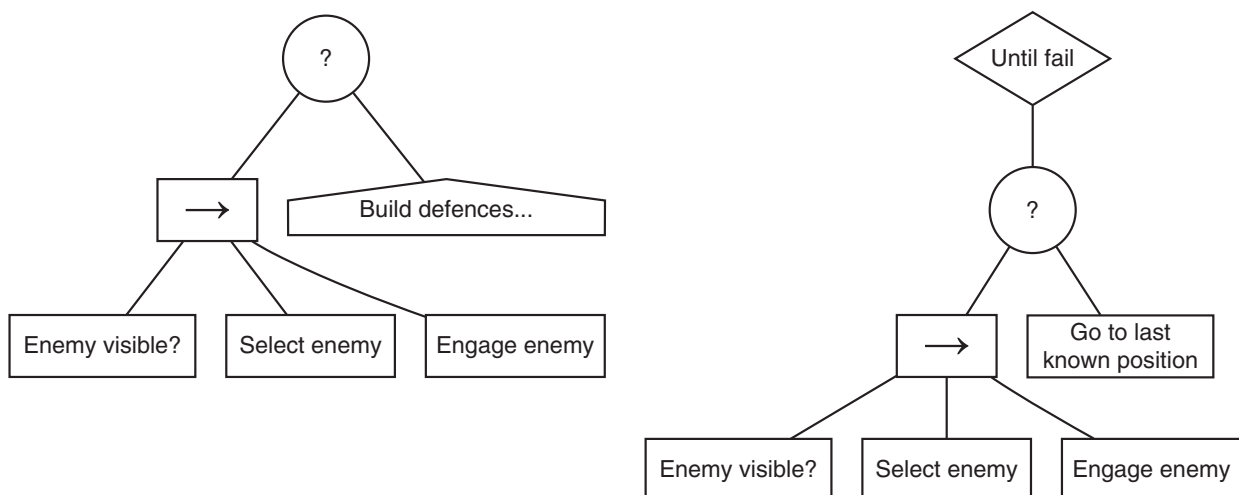
Figure 5.37 Common sub-trees across characters
