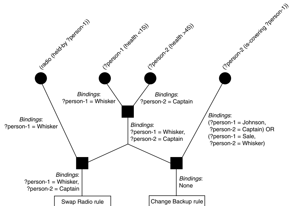
Figure 5.50 The Rete with data
