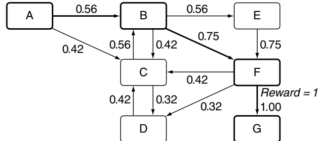
Figure 7.16 A learned state machine
