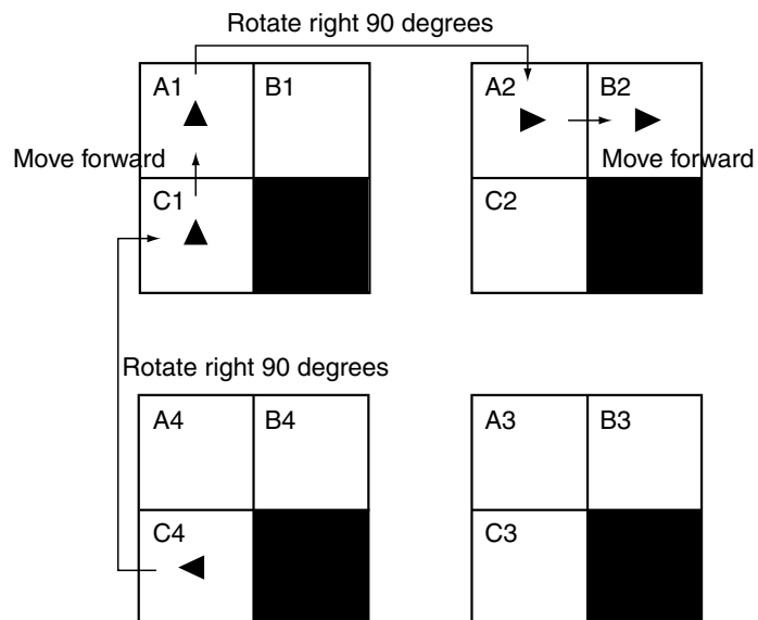
Figure 4.35 Plan on a non-translational tile graph
