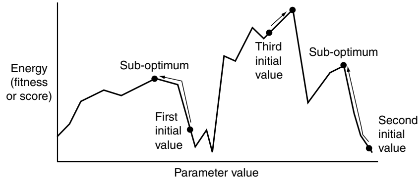
Figure 7.6 Hill climbing multiple trials
