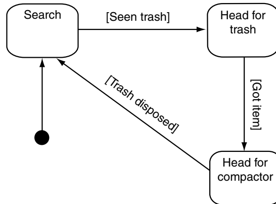
Figure 5.14 The basic cleaning robot state machine
