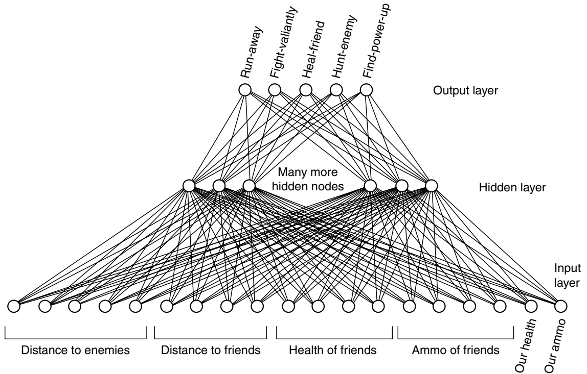
Figure 7.20 Multi-layer perceptron architecture
