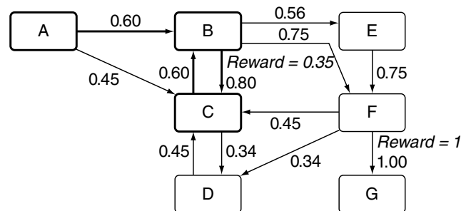
Figure 7.17 A learned machine with additional rewards
