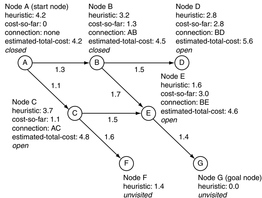
Figure 4.13 A* estimated-total-costs
