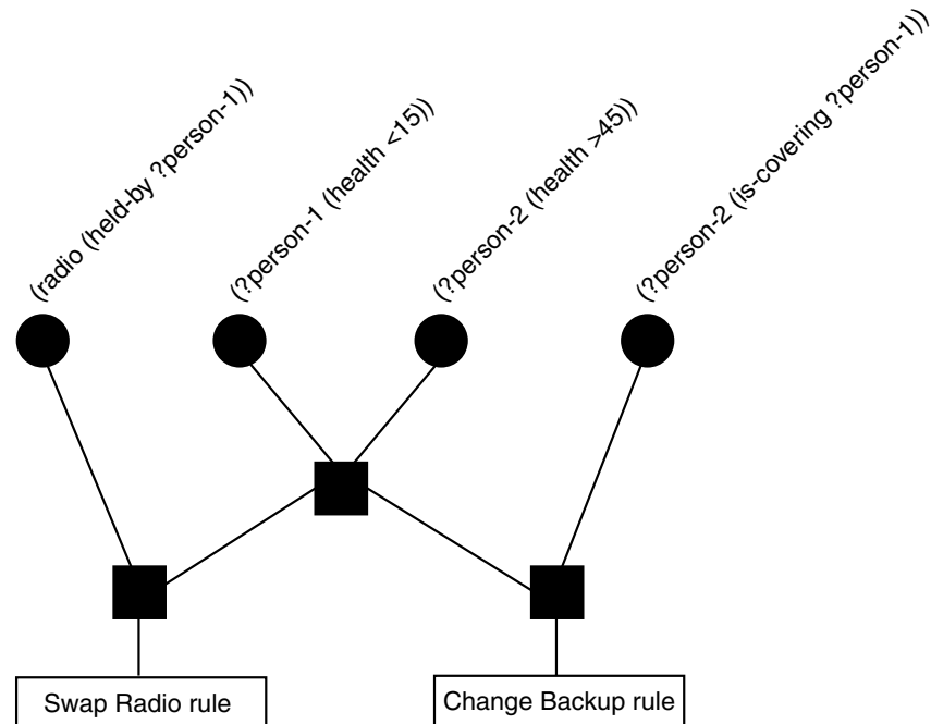
Figure 5.48 A Rete
