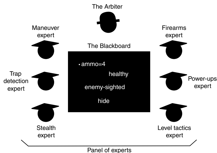
Figure 5.54 Blackboard architecture
