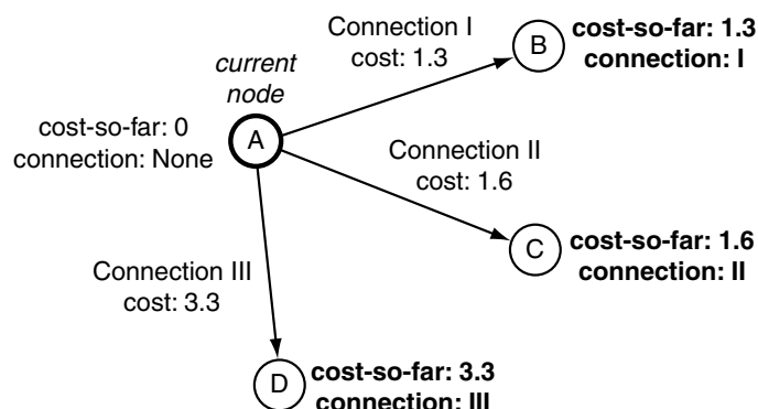
Figure 4.8 Dijkstra at the first node
