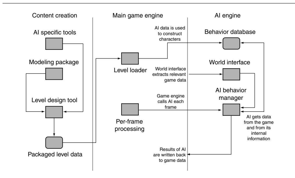
Figure 2.2 AI schematic
