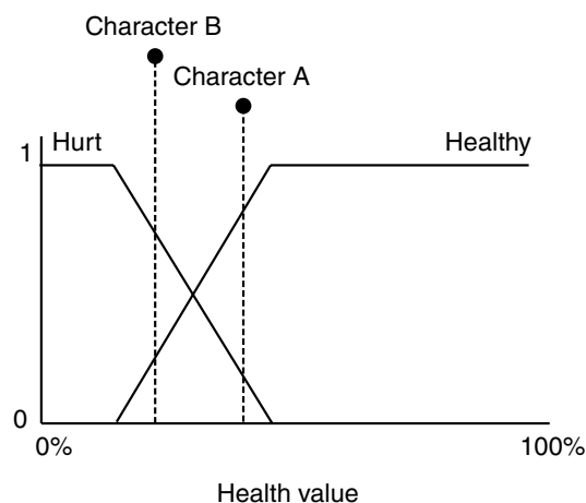
Figure 5.38 Membership functions
