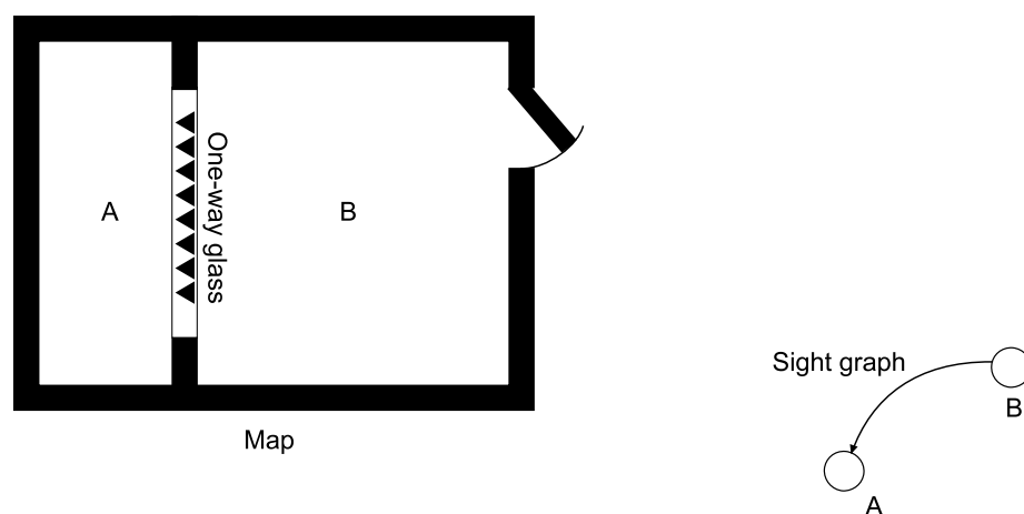
Figure 10.6 Sense graph for one-way glass
