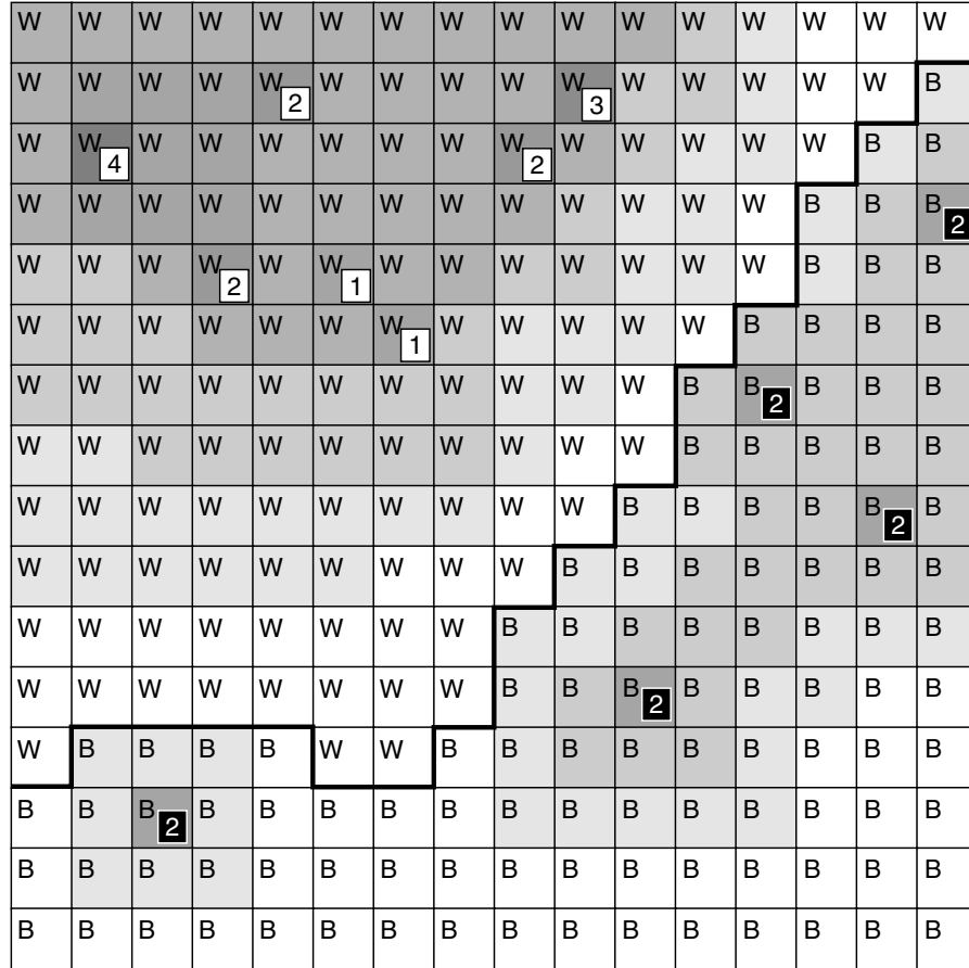
Figure 6.10 An example influence map
