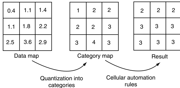
Figure 6.19 Updating a cellular automaton
