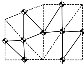
Figure 4.32 Portal representation of a navigation mesh
