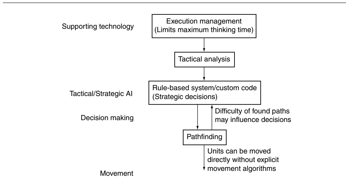
Figure 12.7 AI architecture for turn-based strategy games
