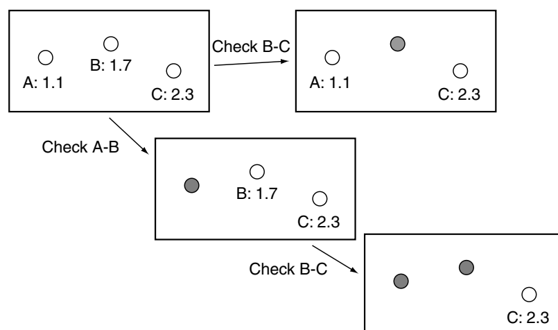
Figure 6.9 Order dependence in condensation checks
