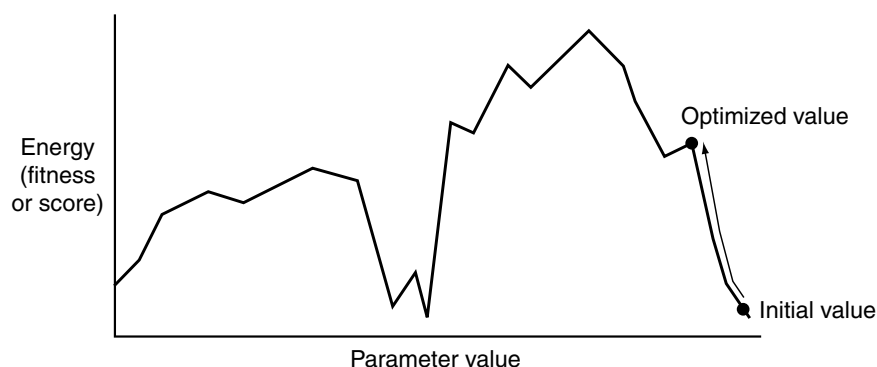
Figure 7.3 Non-monotonic fitness landscape with sub-optimal hill climbing
