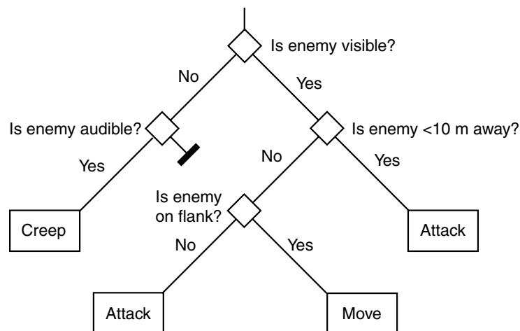
Figure 7.9 A decision tree
