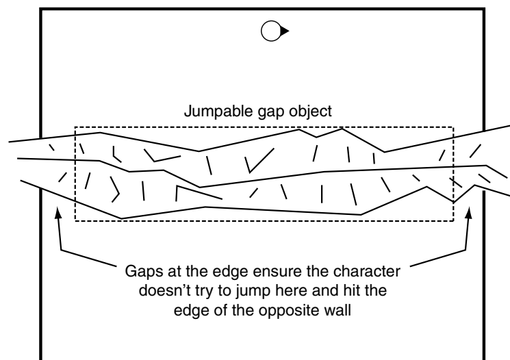
Figure 3.53 A one-direction chasm jump
