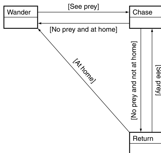
Figure 13.3 The simple behavior of a single predator
