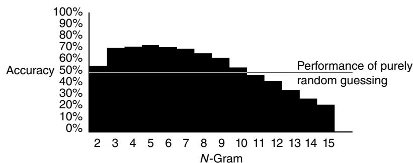
Figure 7.7 Different window sizes
