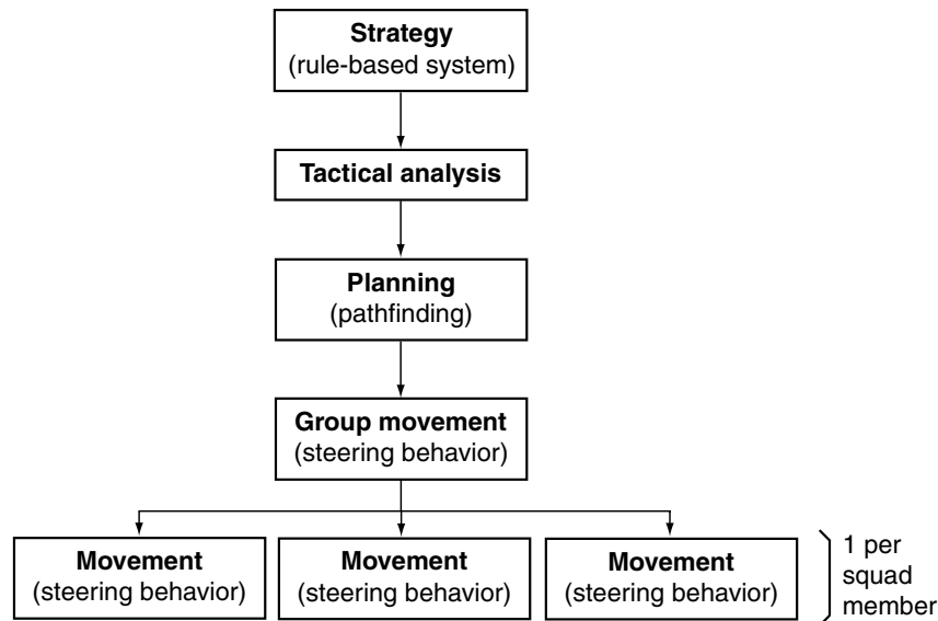
Figure 6.23 An example of multi-tier AI
