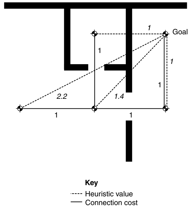
Figure 4.17 Euclidean distance heuristic
