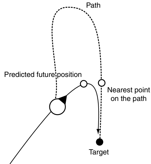
Figure 3.17 Vanilla and predictive path following
