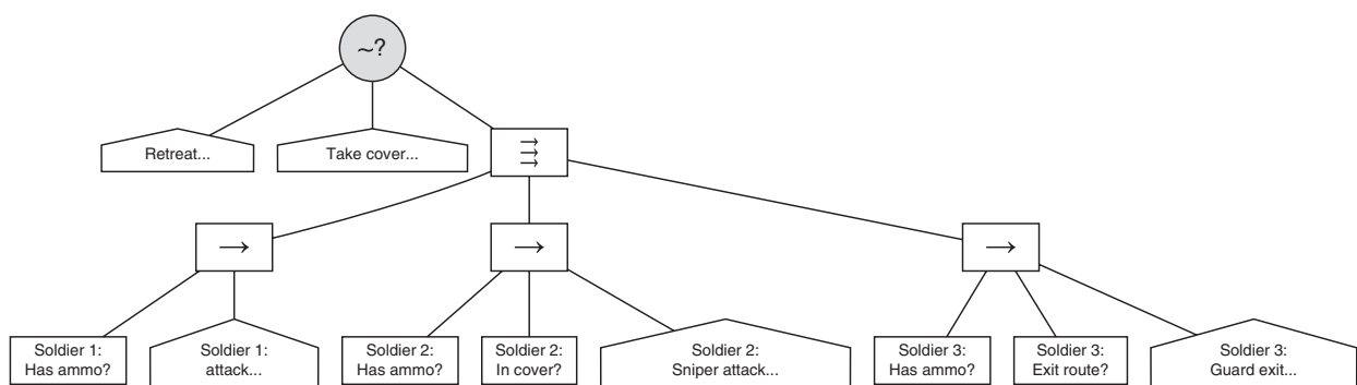
Figure 5.31 Using Parallel to implement group behavior
