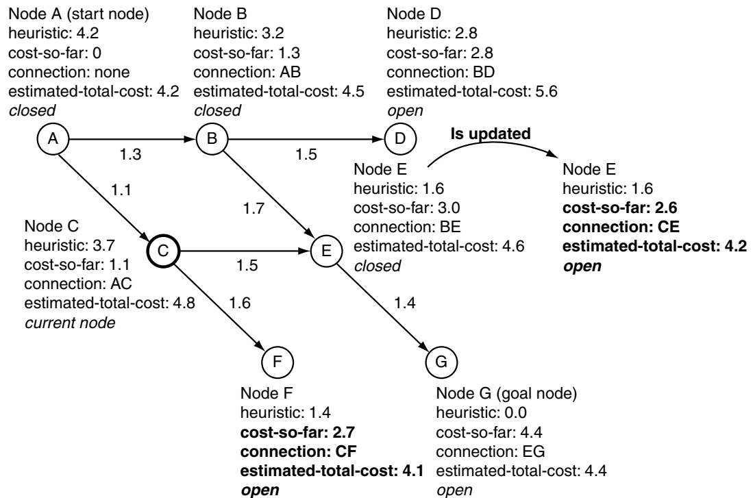
Figure 4.14 Closed node update
