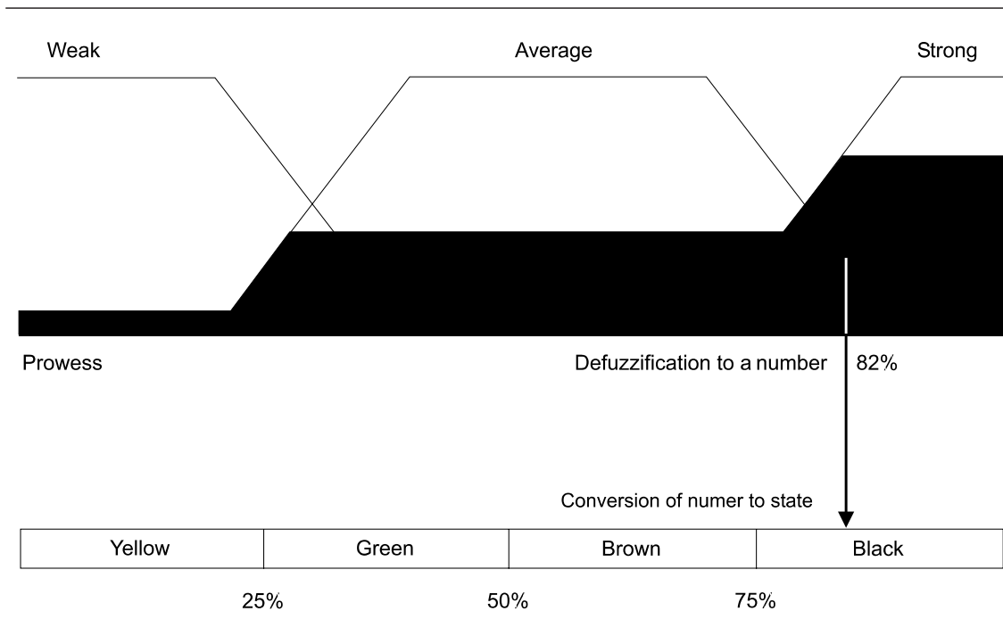
Figure 5.43 Enumerated defuzzification in a range
