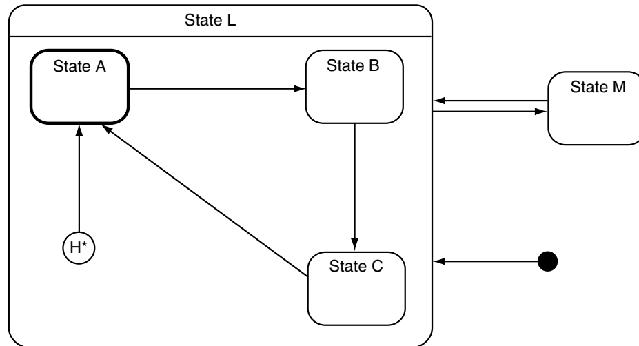
Figure 5.18 Current state in a hierarchy
