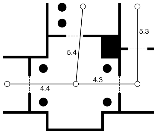
Figure 4.5 Weighted graph overlaid onto level geometry
