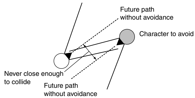
Figure 3.21 Two in-cone characters who will not collide
