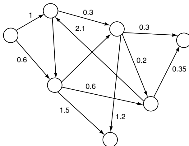
Figure 4.6 A directed weighted graph
