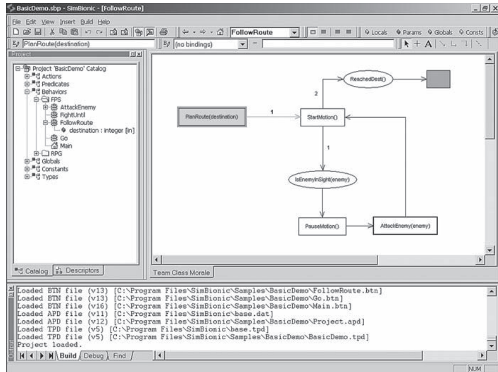
Figure 11.5 The SimBionic editor screen
