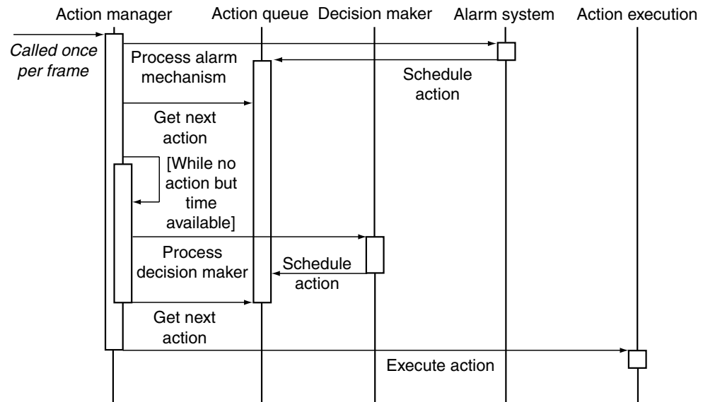
Figure 5.57 The action manager in context
