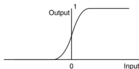
Figure 7.21 The sigmoid threshold function
