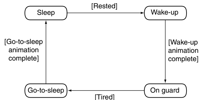
Figure 5.56 State machine with transition states
