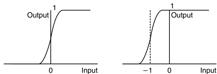
Figure 7.22 Bias and the sigmoid basis function
