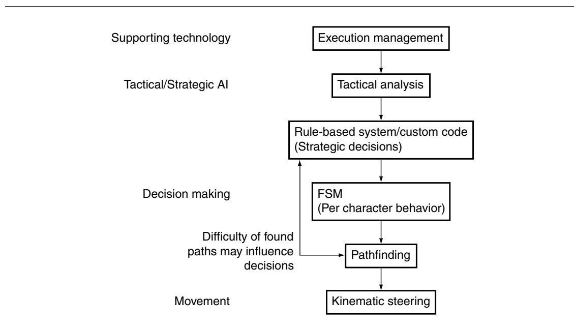
Figure 12.5 AI architecture for RTS games
