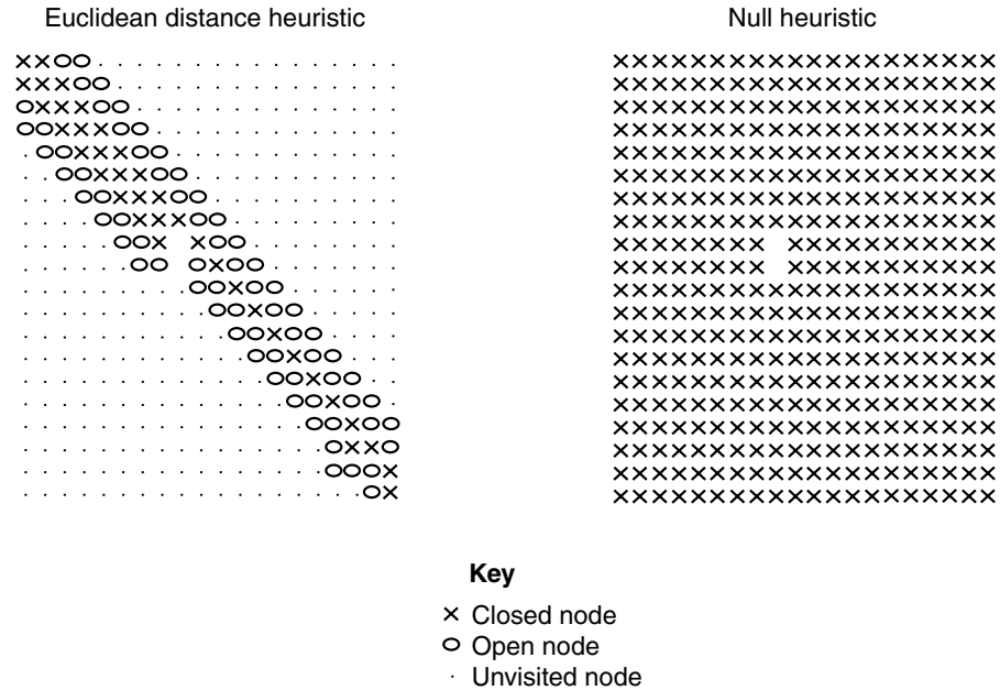
Figure 4.21 Fill patterns outdoors
