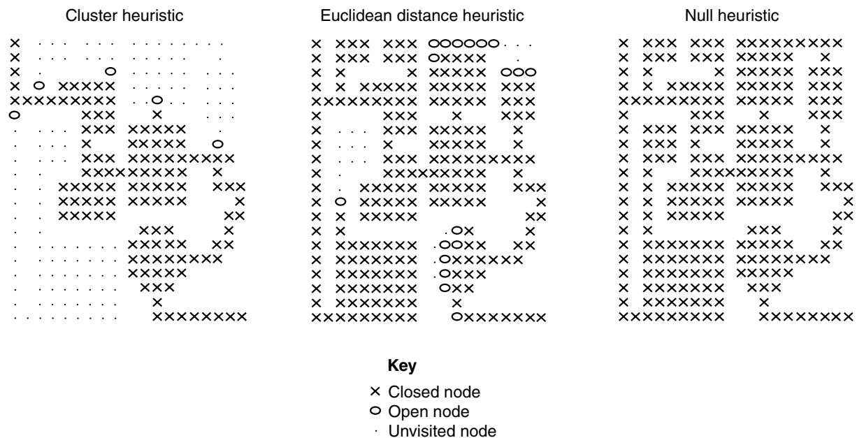
Figure 4.20 Fill patterns indoors
