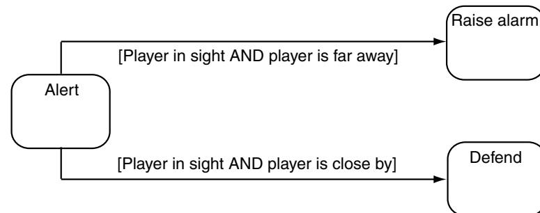
Figure 5.21 State machine without decision tree transitions
