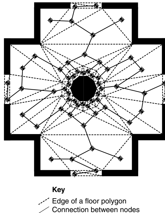
Figure 4.29 Polygonal mesh graph
