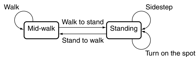
Figure 4.52 Example of an animation state machine
