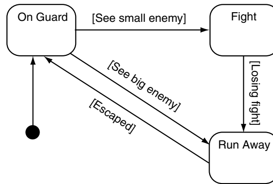
Figure 5.13 A simple state machine
