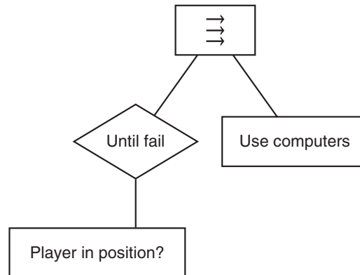
Figure 5.33 Using Parallel to keep track of Conditions
