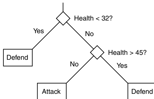
Figure 7.11 Two sequential decisions on the same attribute
