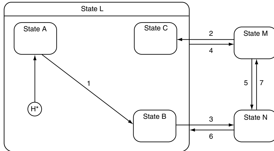
Figure 5.19 Hierarchical state machine example
