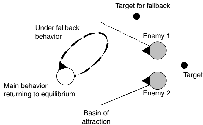
Figure 3.38 Priority steering avoiding unstable equilibrium
