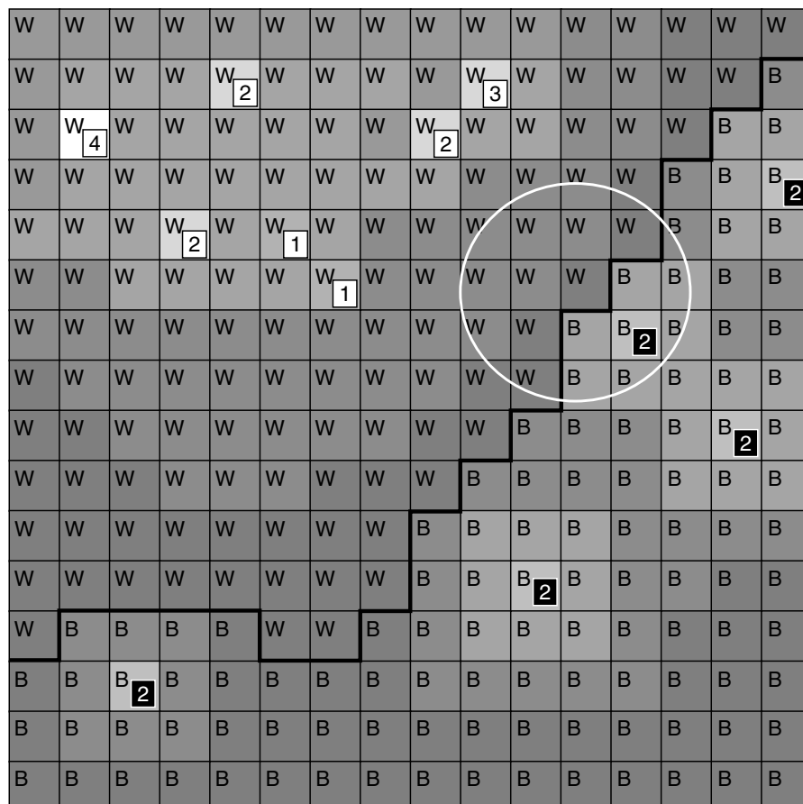
Figure 6.11 The security level of the influence map
