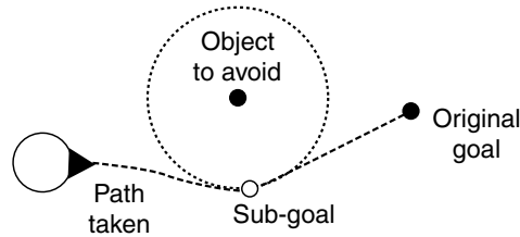
Figure 3.42 Collision avoidance constraint
