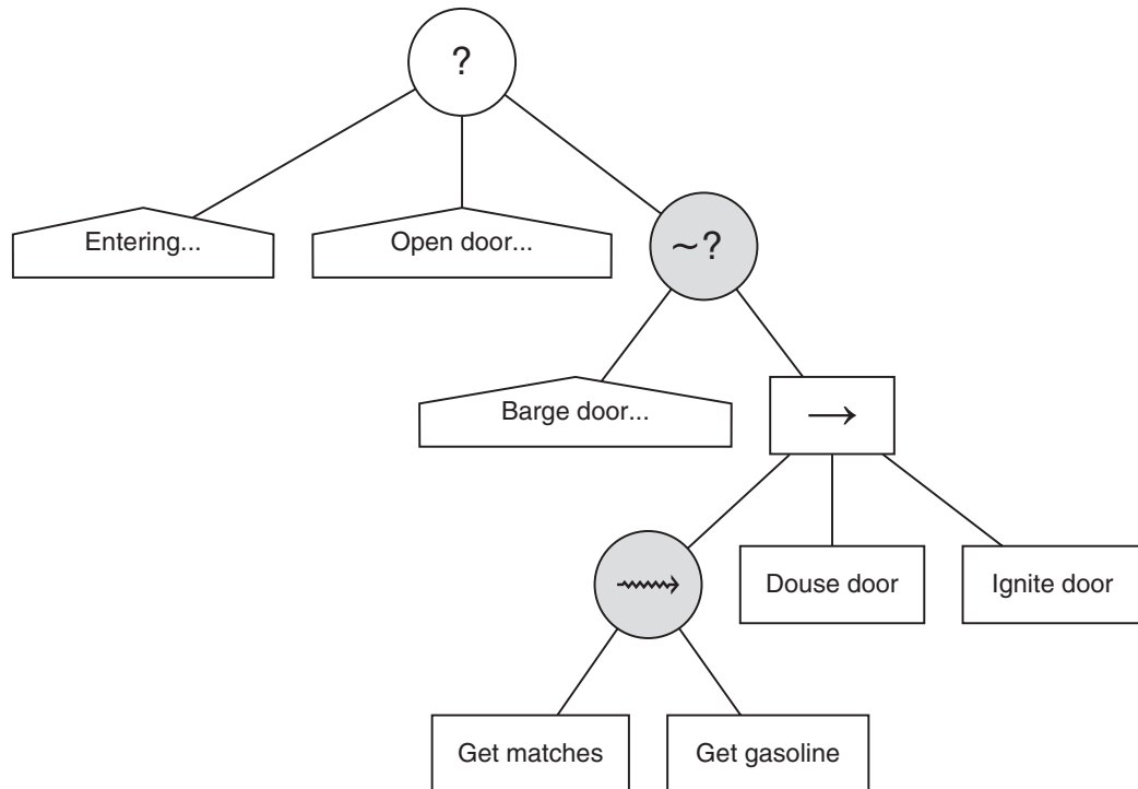
Figure 5.28 Example behavior tree with partial ordering
