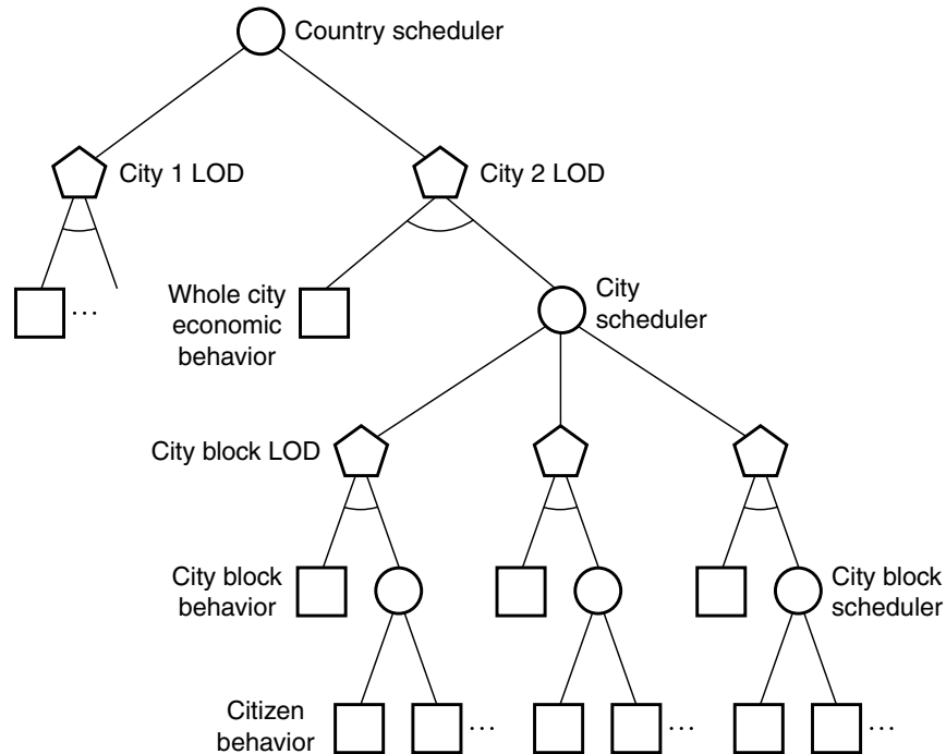
Figure 9.6 Hierarchical LOD algorithms
