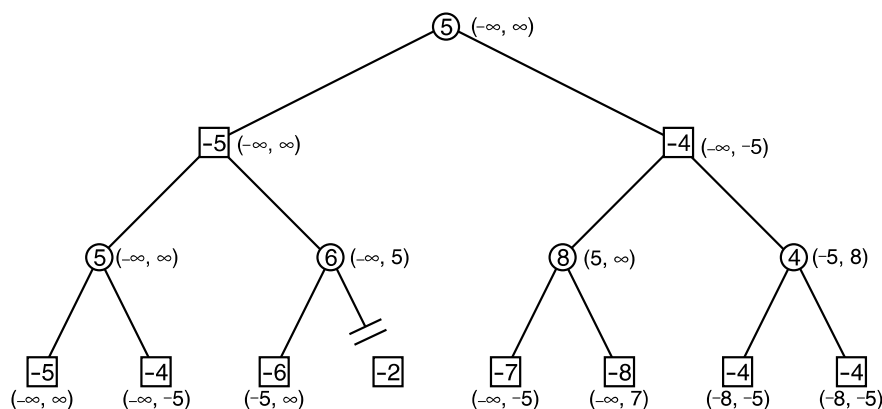
Figure 8.10 AB negamax calls on a game tree
