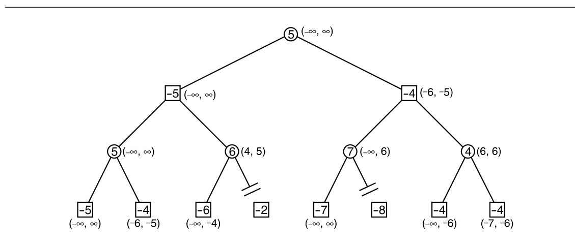
Figure 8.11 The game tree with negascout calls
