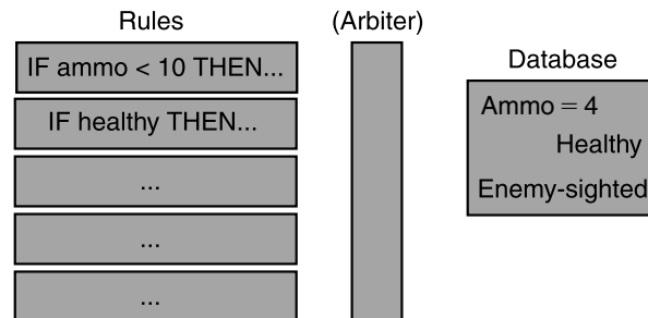
Figure 5.46 Schematic of a rule-based system
