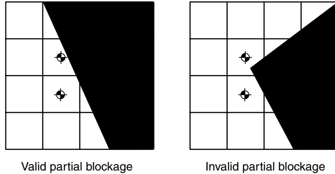
Figure 4.23 Tile-based graph with partially blocked validity
