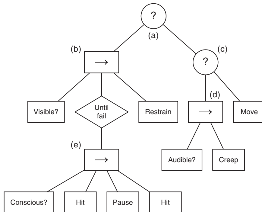
Figure 5.29 Example behavior tree
