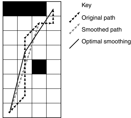
Figure 4.36 Smoothed path with optimal smoothing indicated
