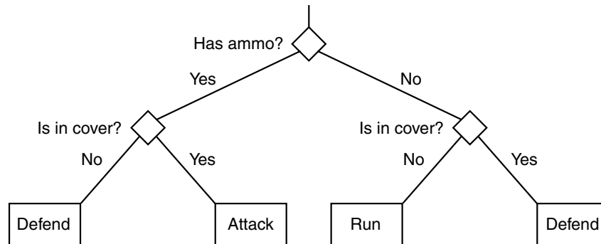
Figure 7.14 Decision tree mid-ID4
