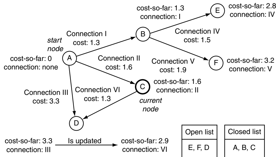
Figure 4.10 Open node update
