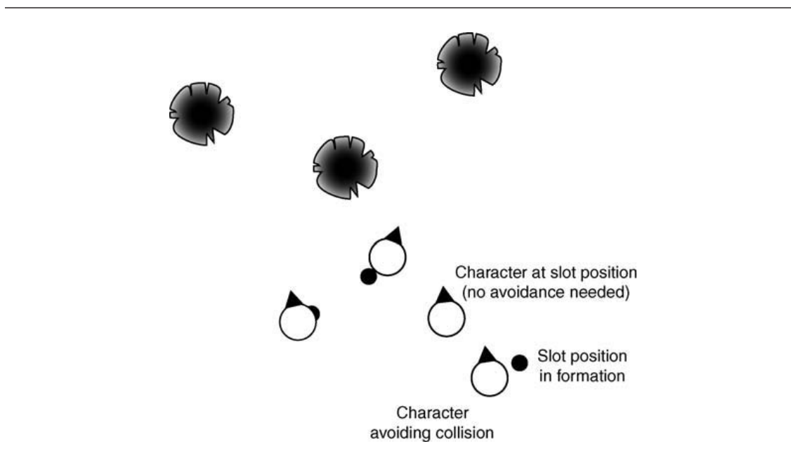
Figure 3.57 Two-level formation motion in a V
