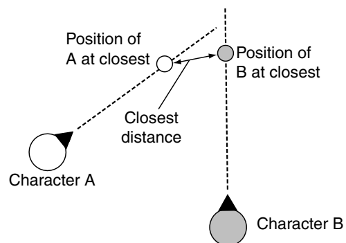
Figure 3.23 Collision avoidance using collision prediction
