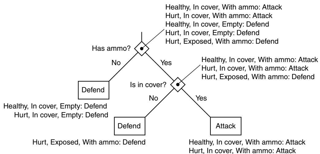
Figure 7.12 The example tree in ID4 format
