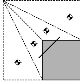
Figure 4.31 Non-interpolation of the navigation mesh
