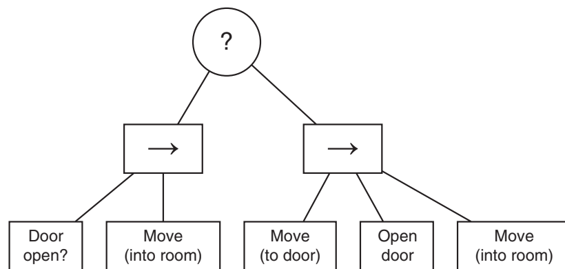
Figure 5.25 A behavior tree with composite nodes
